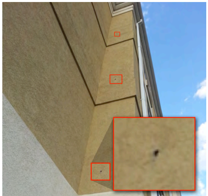
Small holes in the EIFS; if left unrepaired, this can result in water infiltration and trapped moisture.
